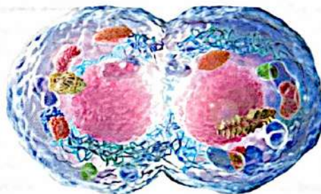
DIVIDING CELL
